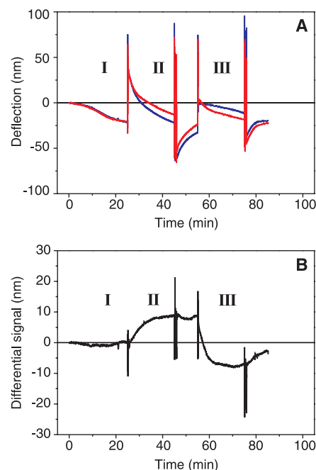
Fig. 3. Hybridization experiment using two cantilevers functionalized with the sequences 5'-TGCAGTAGACCT-3' (12-mer oligonucleotide), the complementary 16-mer oligonucleotide (1 ml, 400 nM in HB) was injected (interval II). The liquid cell was purged 20 min later with 3 ml of HB. Then, the complementary 12-mer oligonucleotide (1 ml, 400 nM in HB) was injected (interval III). The liquid cell was again purged 20 min later with 3 ml of HB. (A) Absolute deflection versus time of two individual cantilevers covered with the 16-mer (red) and the 12-mer (blue) oligonucleotide. (B) Corresponding differential signal.
